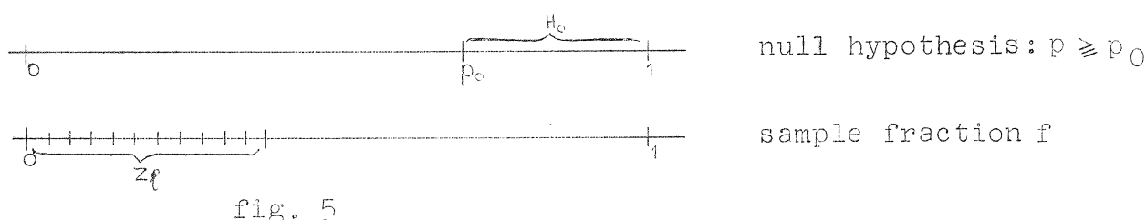
Left one-sided test of the null-hypothesis p \geq p_0
