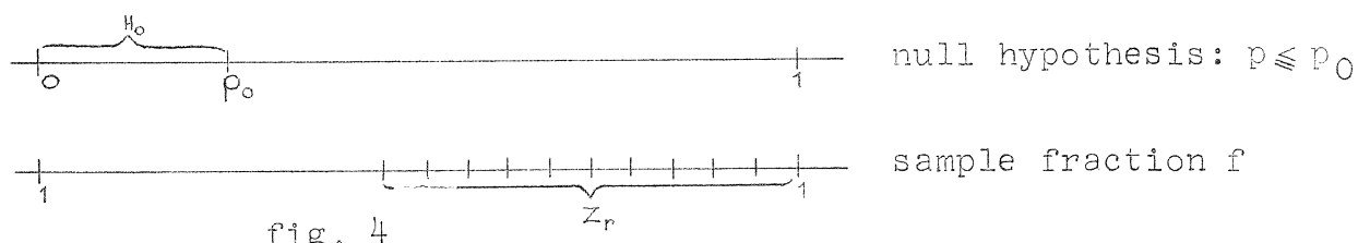
Right one-sided test of the hypothesis p \leq p_0
